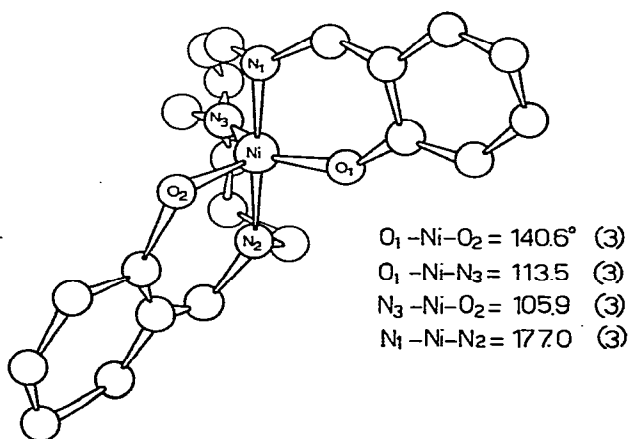
Fig. 5. The stereochemistry of Ni(SalMedpt) (from Ref. 23).
